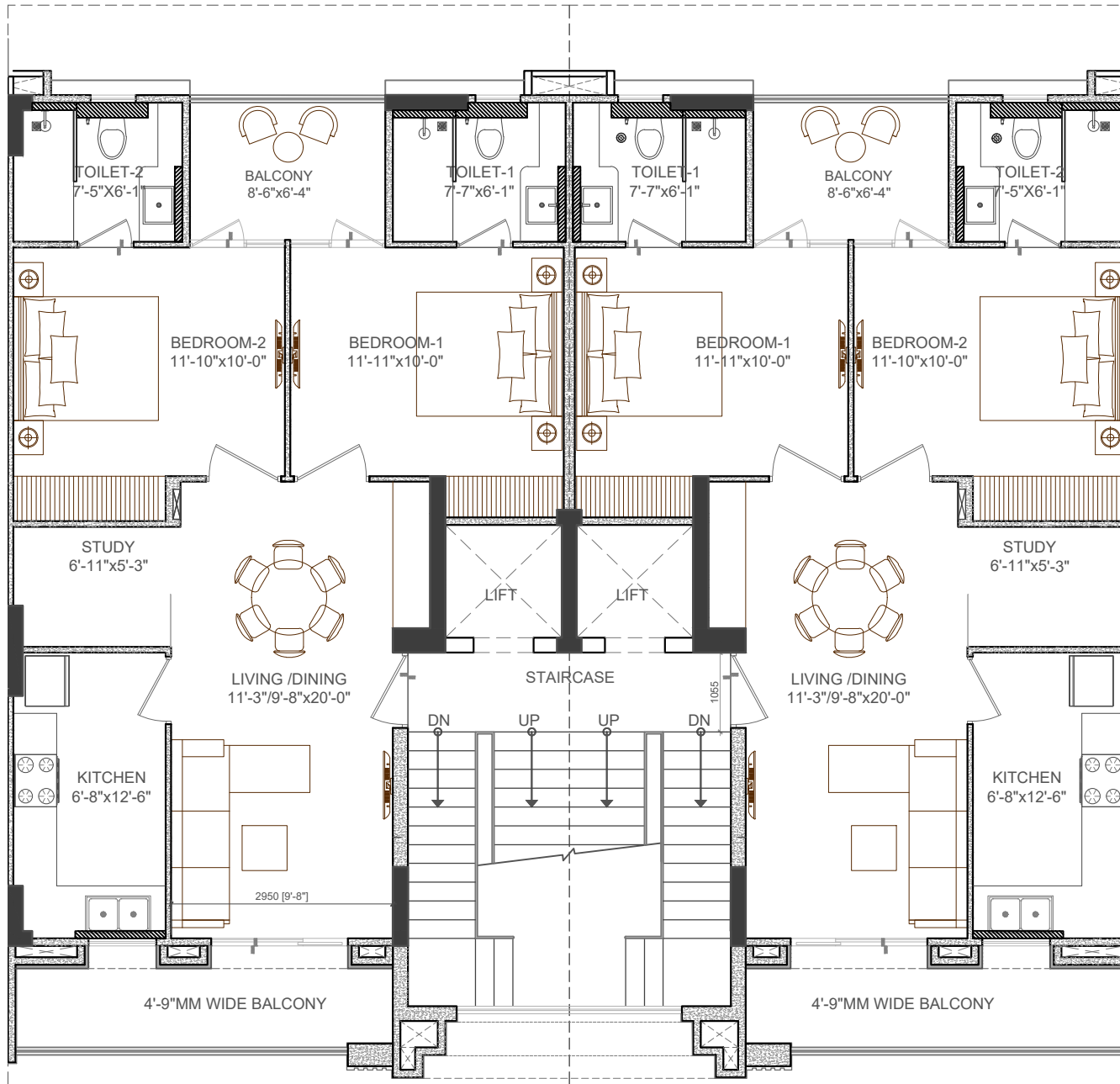
TYPICAL FLOOR PLAN
